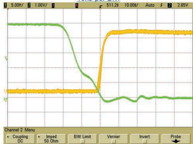
GREEN TRACE: TTL SIGNAL YELLOW TRACE: RF SIGNAL
